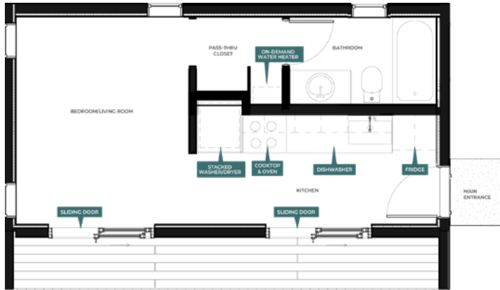
Exterior Dimensions: 25'W x 16'D X 10'2"H
